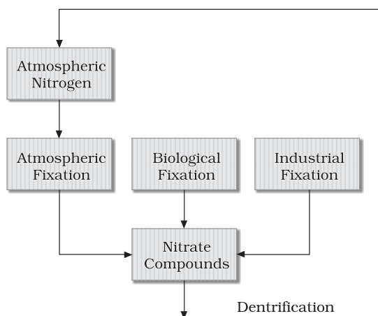
Figure 15.3 : Nitrogen Cycle
