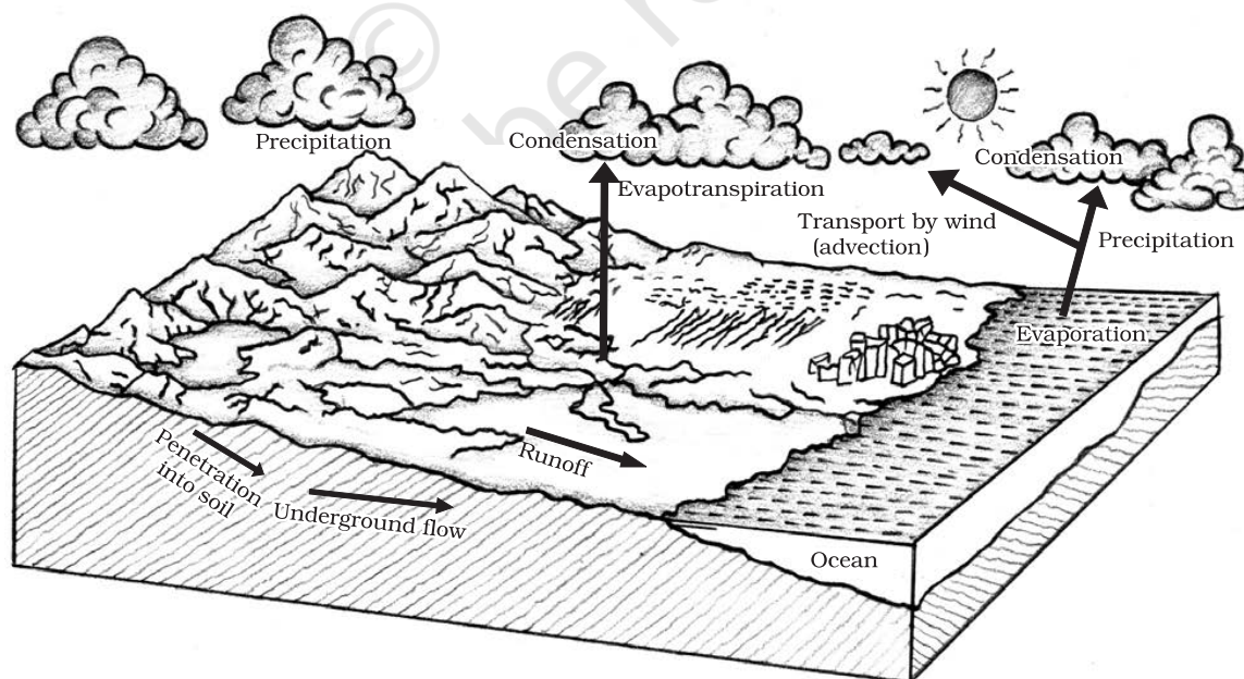
Figure 13.1 : Hydrological Cycle
