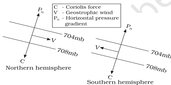
Figure 10.4 : Geostrophic Wind
