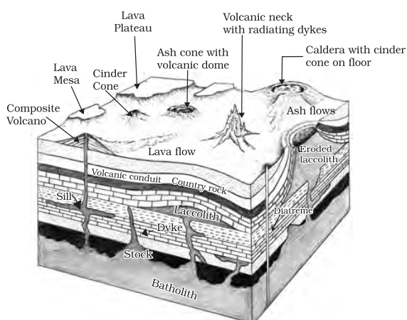
Figure 3.5 : Volcanic Landforms
