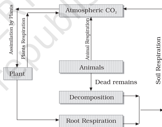
Figure 15.2 : Carbon Cycle
