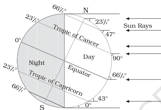
Figure 9.1 : Summer Solstice
