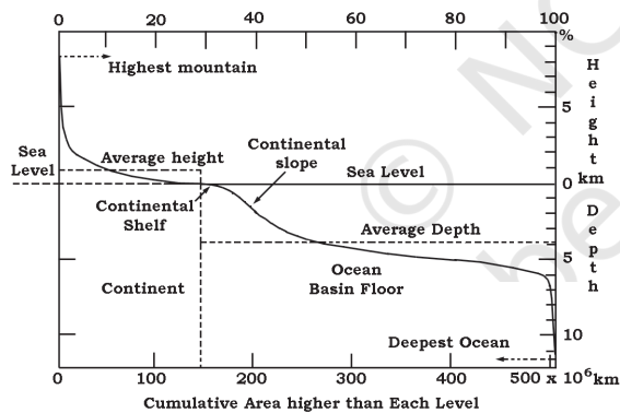
Figure 4.1 : Ocean Floor
