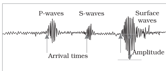
Figure 3.1 : Earthquake Waves
