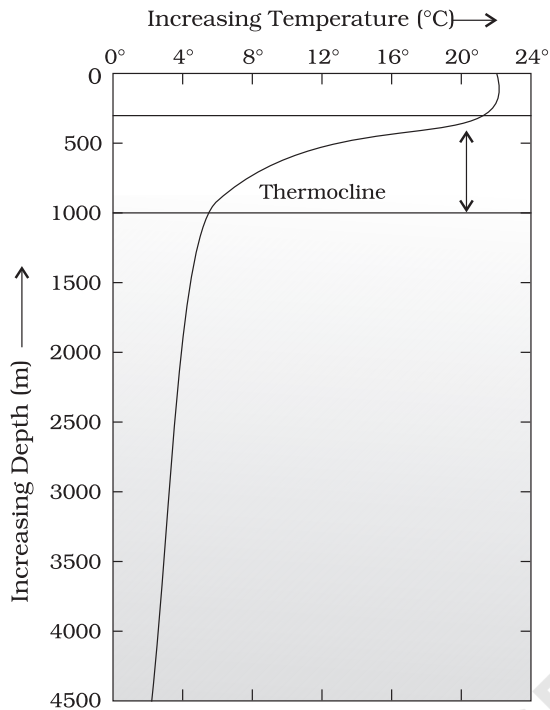
Figure 13.3 : Thermocline
