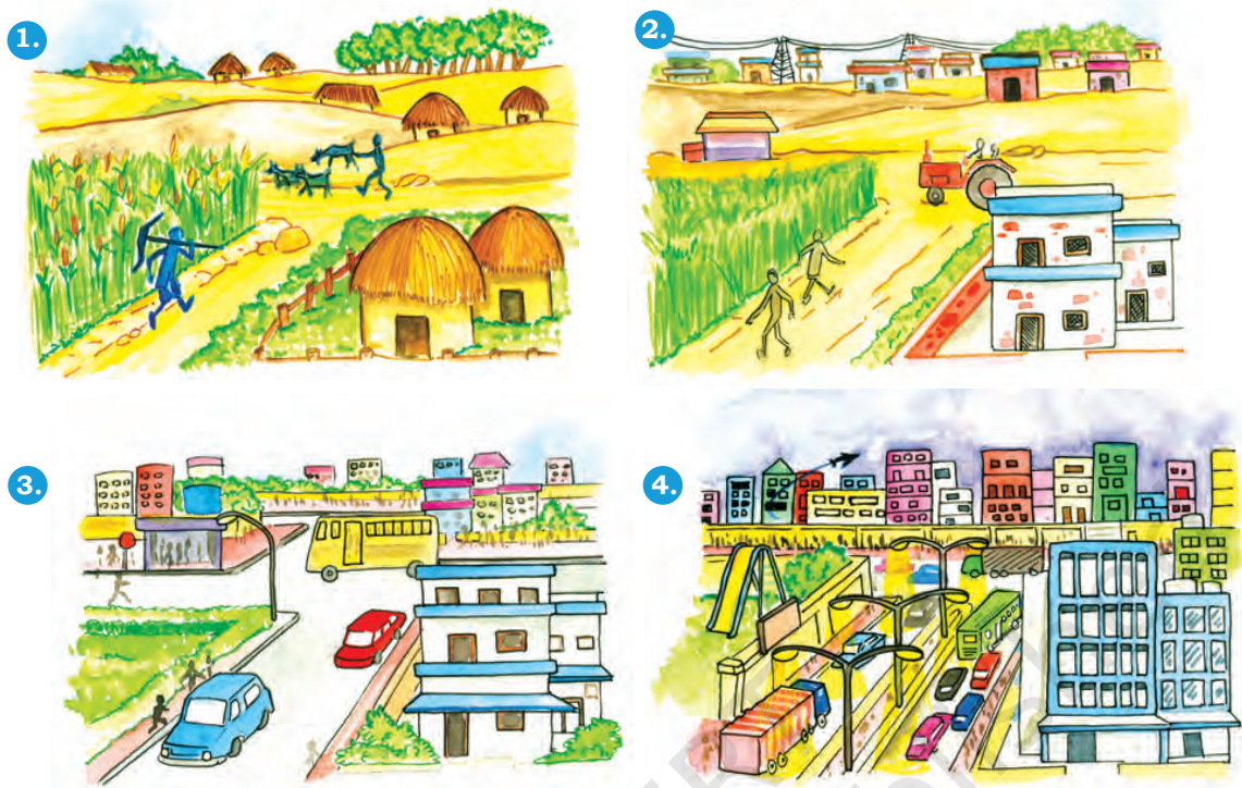
Fig. 2.2: Change in land use over time
