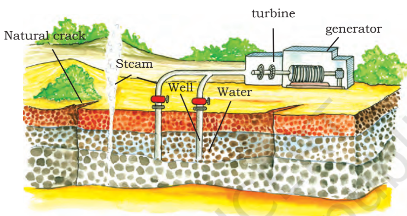
Fig. 3.19 : Geothermal Energy
