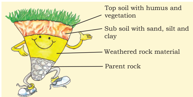
Fig. 2.3: Soil Profile
