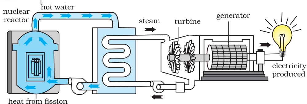
Fig. 3.17 : Nuclear Energy
