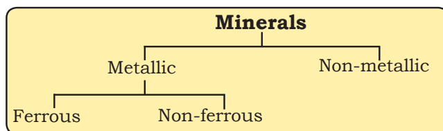
Fig. 3.2: Classification of Minerals
