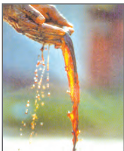
Fig 3.11: Crude Oil
