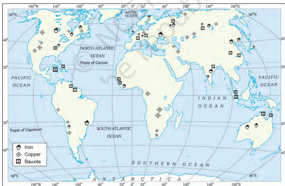
Fig. 3.5: World: Distribution of Iron, Copper and Bauxite
