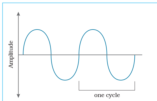
Fig.5.3 : Sound Waves
